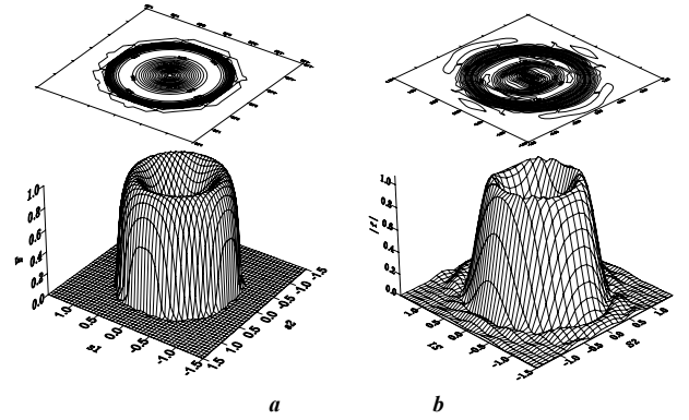
Figure 4. The prescribed (a) and synthesized (b) DPs
