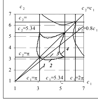
Figure 1. The possible branching lines of solutions of system of (14) for F(s_1, s_2) \equiv 1
