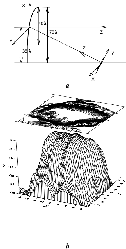
Figure 15. Synthesized contour DP based on the hybrid reflector antenna
