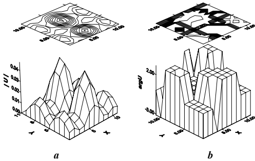
Figure 10. Optimal distributions of amplitude (a) and phase (b) of currents in the array \mathbf{u}
