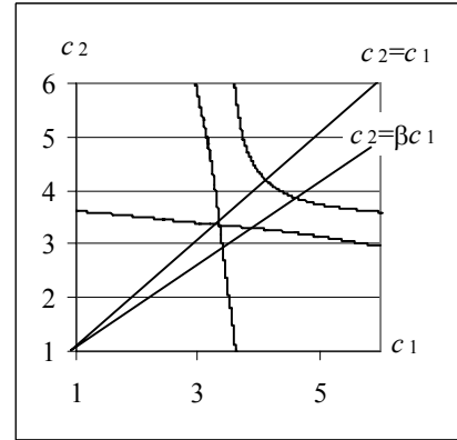
Figure 2. The possible branching lines of solutions of system of (14) for F(s_1, s_2) , which is defined by (36)
