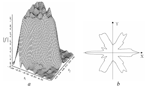
Figure 12. Synthesis of DP with triangular contour: a — synthesized DP with quasi-triangular contour, b — optimal shape of aperture
