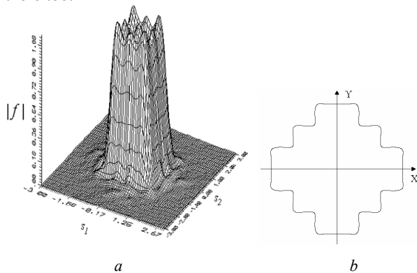
Figure 11. Synthesis of DP with square contour: a — synthesized DP with square contour, b — the optimal shape of aperture
