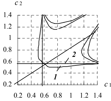
Figure 7. The possible branching lines of solutions of (53) for F(s_1, s_2) = |\sin(\pi s_1)| \cdot |\sin(\pi s_2)|
